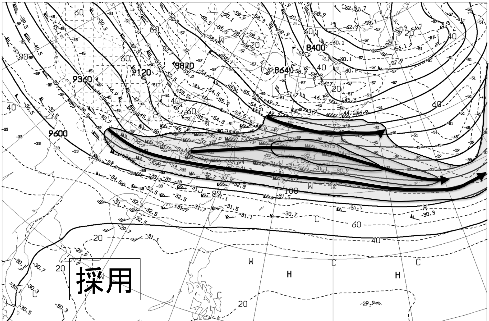
ANALYSIS 300hPa: HEIGHT(M), TEMP(°C), ISOTACH(KT)
